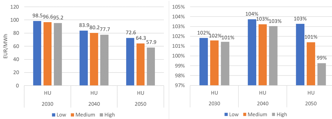
Figure 10: Wind Market value in Hungary in the three analysed scenarios, €/MWh (left) and % compared to baseload prices
