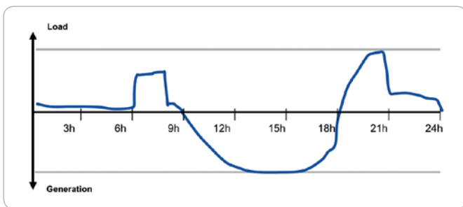
Power profile without the Smart Operator
